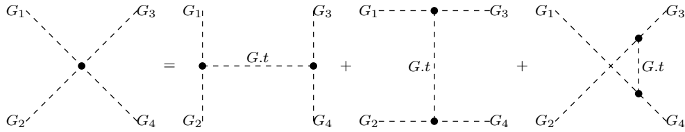
Figure 13: Splitting of four-gluon vertex
