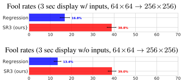
Figure 7: ImageNet super-resolution fool rates (higher is better, photo-realistic samples yield a fool rate of 50%). SR3 and Regression outputs are compared against ground truth. (top) Subjects are shown low-resolution inputs. (bottom) Inputs are not shown.
