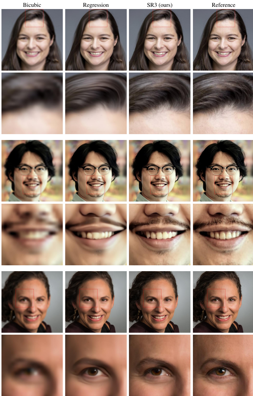
Figure C.1: Additional results of a SR3 model ( 64\times 64 \rightarrow 512\times 512 ), trained on FFHQ, and applied to images outside of the training set. We crop and align these faces to be consistent with FFHQ using the script provided here .
