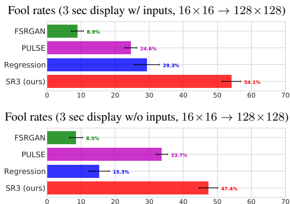
Figure 6: Face super-resolution human fool rates (higher is better, photo-realistic samples yield a fool rate of 50%). Outputs of 4 models are compared against ground truth. (top) Subjects are shown low-resolution inputs. (bottom) Inputs are not shown.
